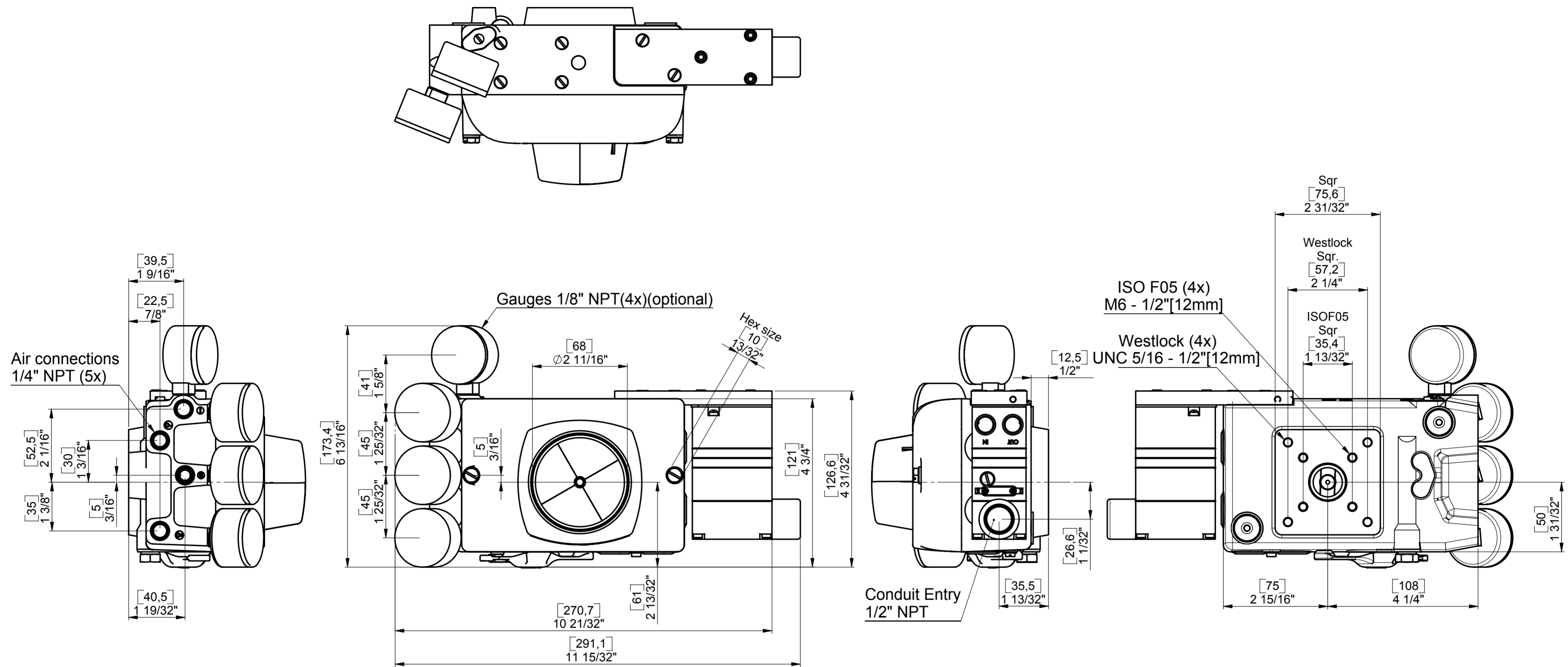
Dimensional Drawing VAC Positioner V200 0/10V IP-Fairchild TA7800
