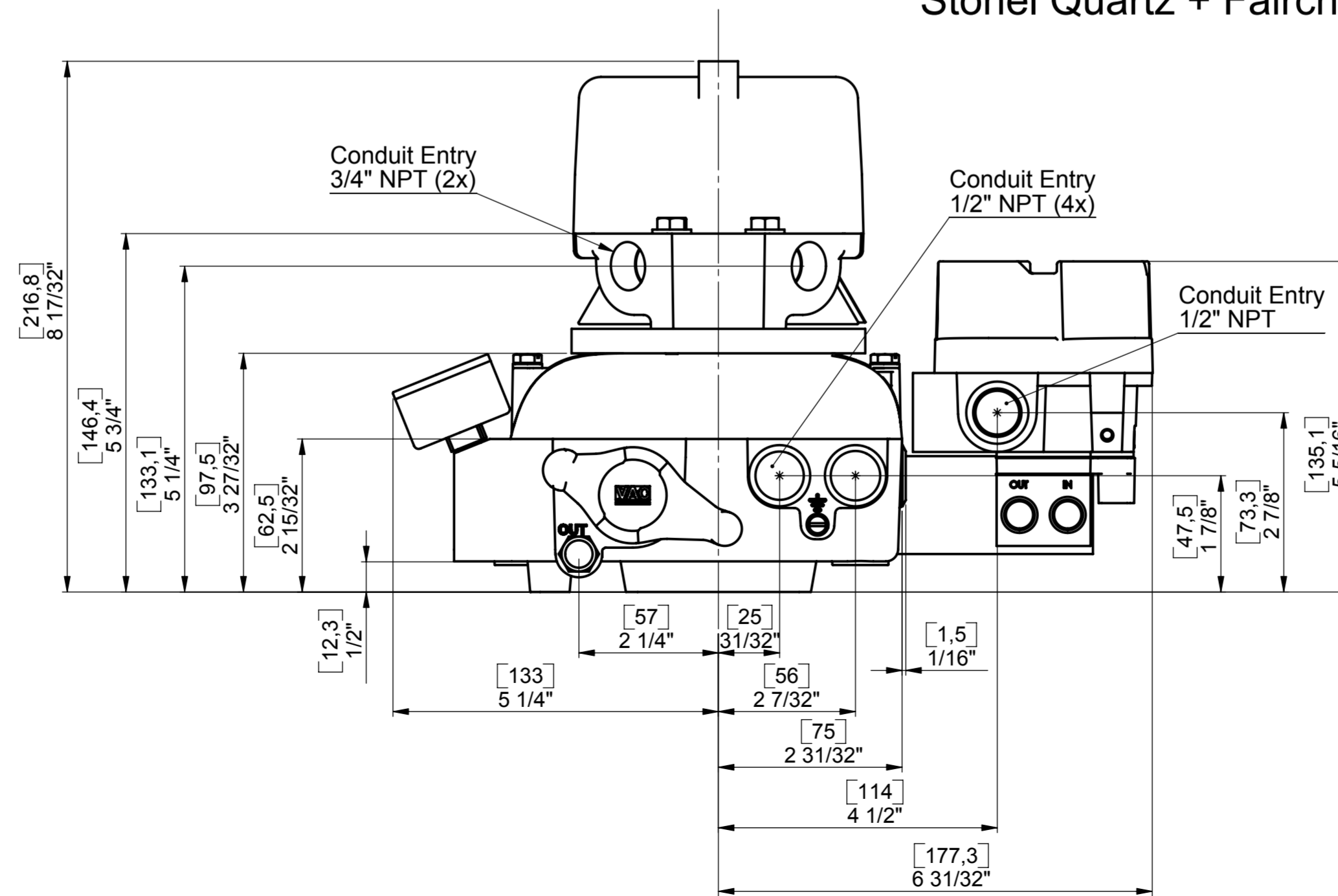
Dimensional Drawing VAC Positioner V200 Stonel Quartz + Fairchild X17800P
