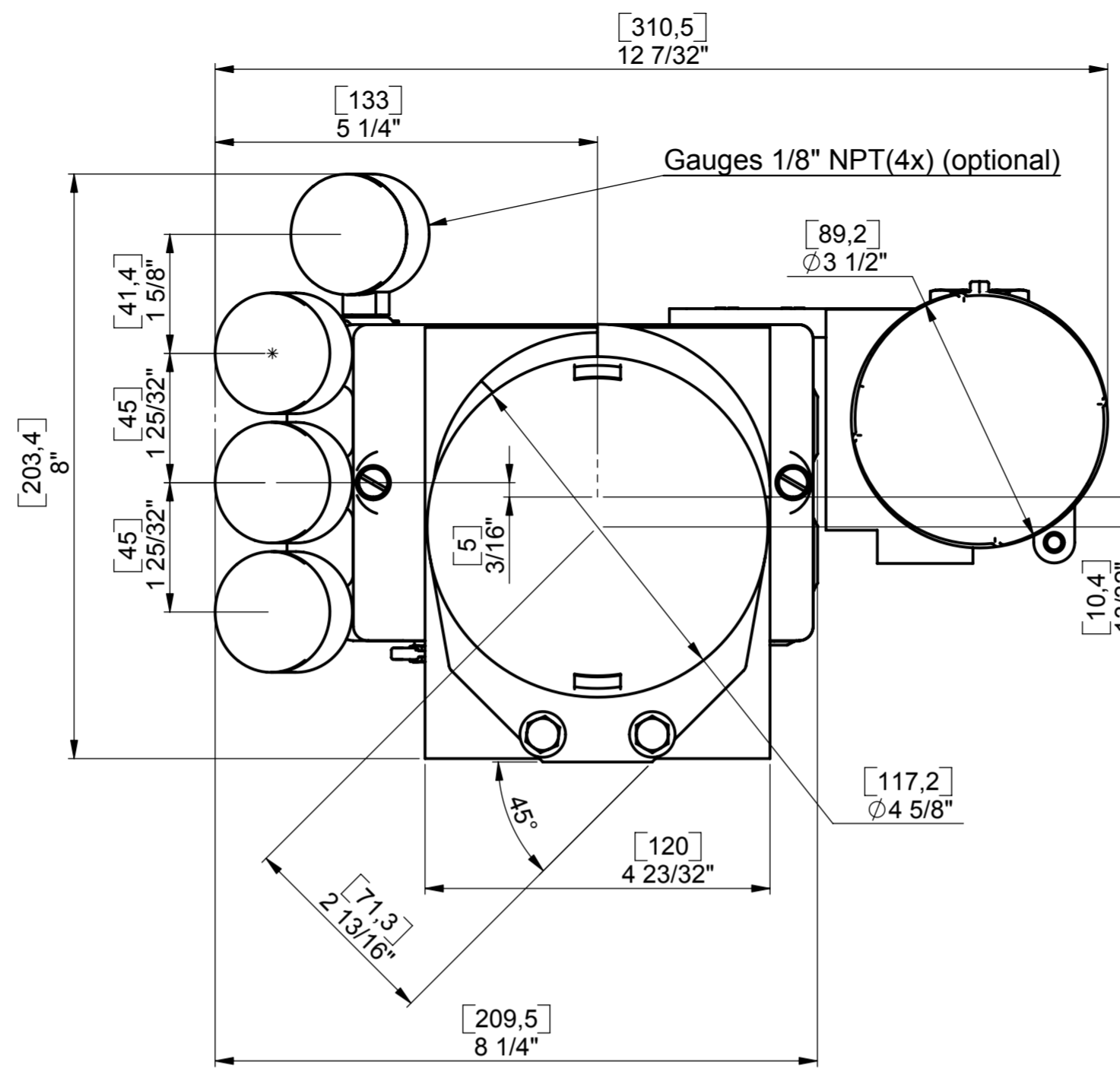
Dimensional Drawing VAC Positioner V200 Stonel Quartz + Fairchild X17800P
