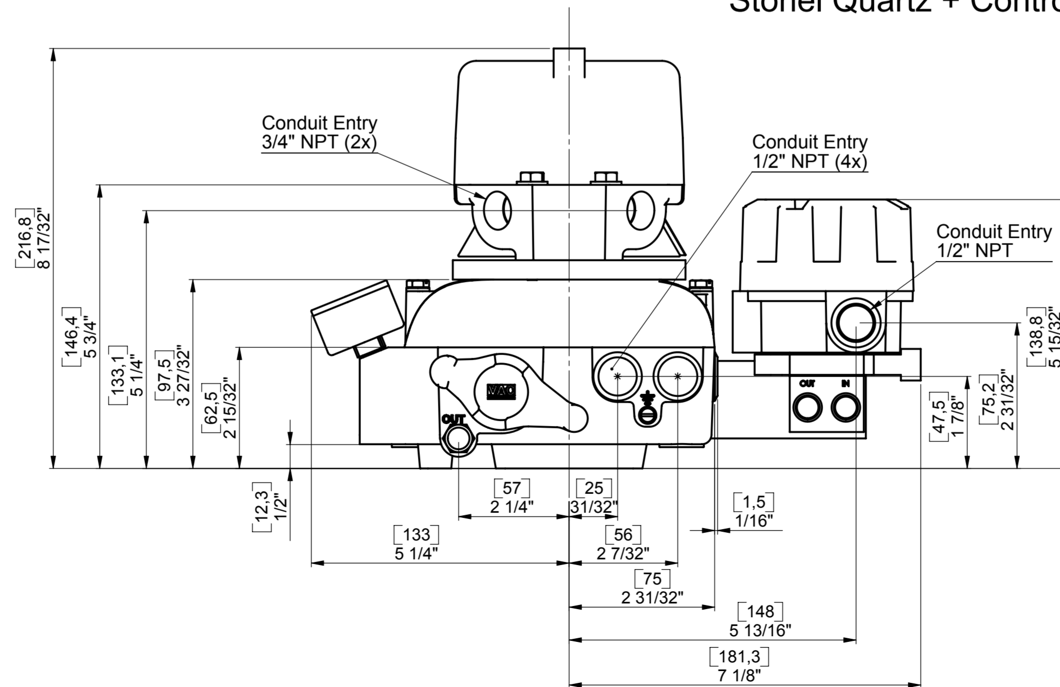
Dimensional Drawing VAC Positioner V200 Stonel Quartz + Control Air 950XP
