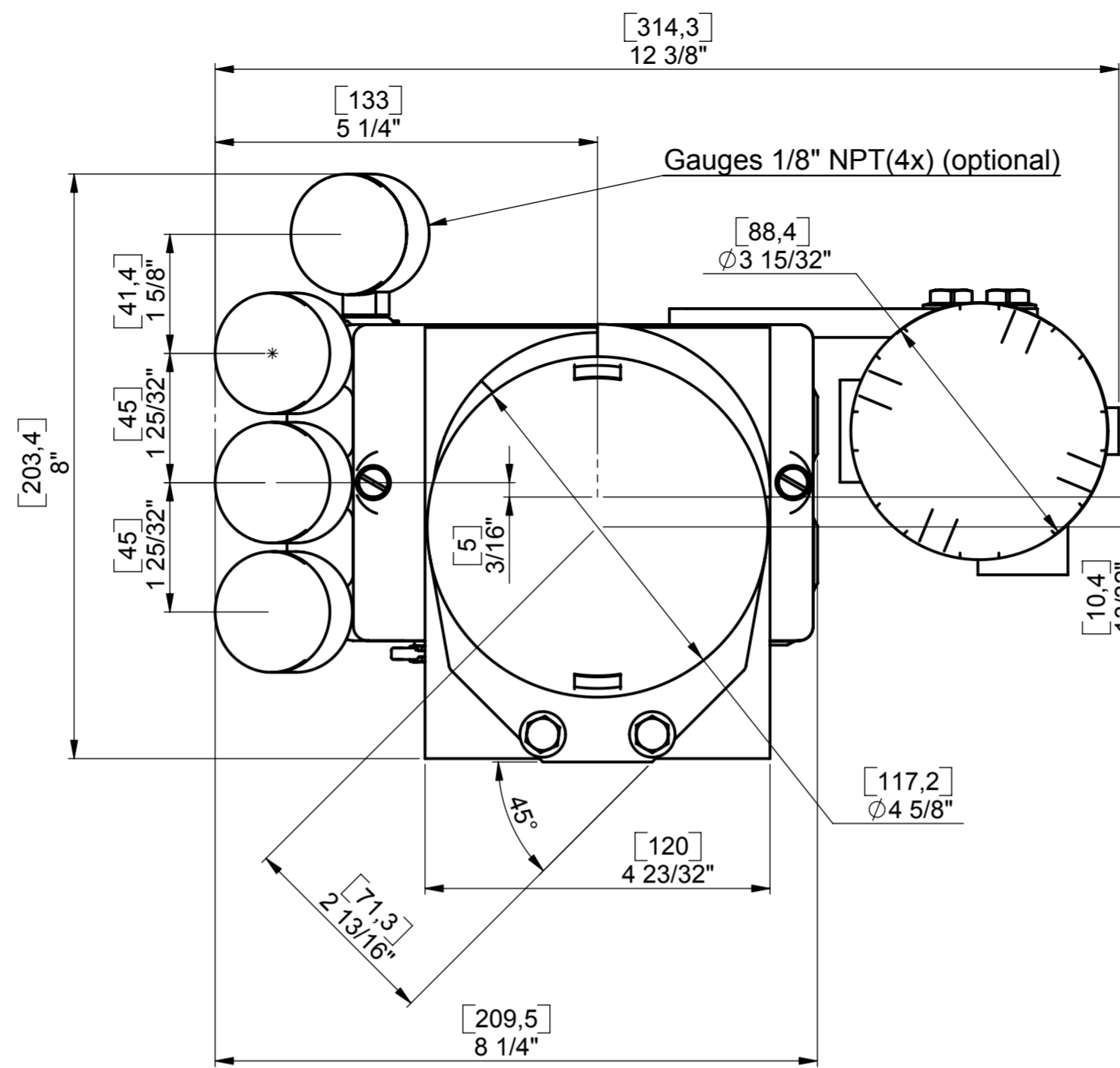
Dimensional Drawing VAC Positioner V200 Stonel Quartz + Control Air 950XP
